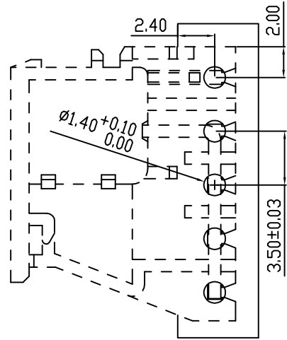
PCB LAYOUT
