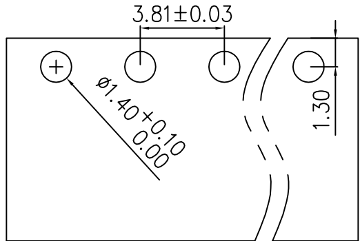
PCB LAYOUT
